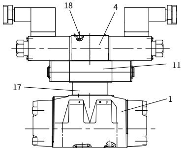
GWEH.../6B2...S...D1型阀装有定比减压阀结构图
