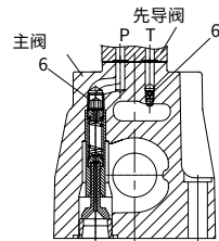
GWEH25.../6B2...型供排结构图
